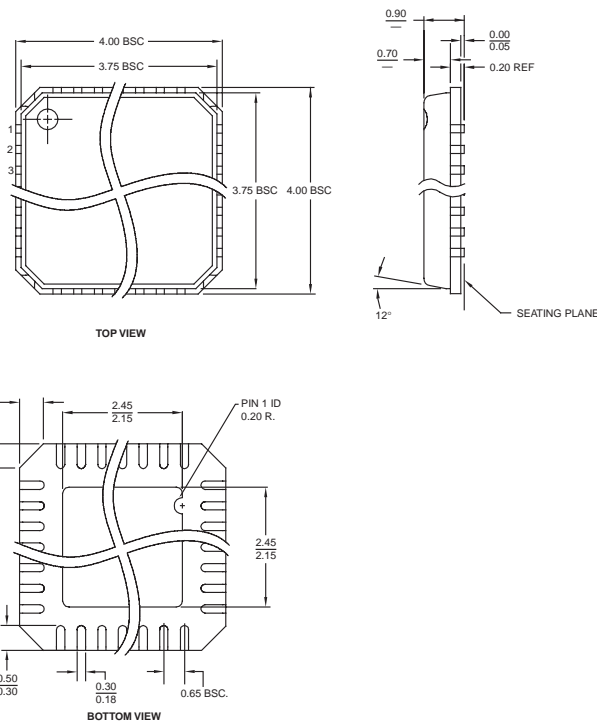
16-Lead MLF™ (ML)
