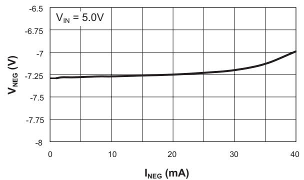
Negative Output Voltage vs. Load Current ( T_A = 25^{\circ}\text{C} )
