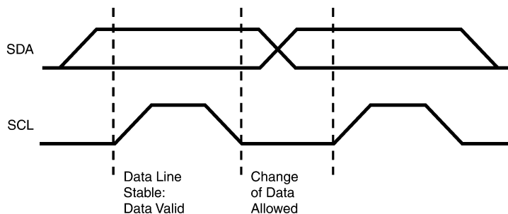
FIGURE 29. Bit Transfer
