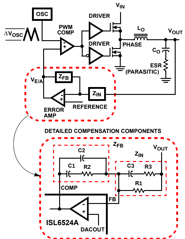
The modulator transfer function is the small-signal transfer function of V_{OUT}/V_{E/A} . This function is dominated by a DC Gain, given by V_{IN}/V_{OSC} , and shaped by the output filter, with a double pole break frequency at F_{LC} and a zero at F_{ESR} .
