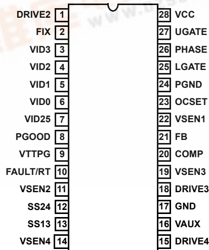
ISL6524A (SOIC) TOP VIEW
