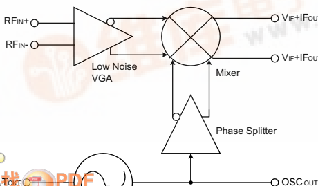
Figure 1: Downconverter Block Diagram
