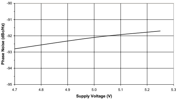
Figure 7: Typical Phase Noise at 10 kHz Offset vs. Supply Voltage ( T_A = +25\text{ }^{\circ}\text{C} , f_{LO2} = 1042\text{ MHz} )
