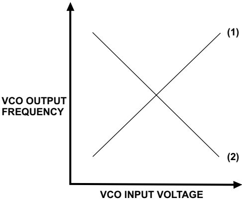
Figure 22: VCO Characteristics
