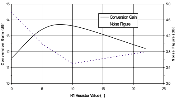
Figure 17: Typical Conversion Gain and Noise Figure vs. LNA/Mixer Current Control Resistor R1 ( T_A = +25\text{ }^{\circ}\text{C} , V_{DD} = +5\text{ V} , f_{LO2} = 1042\text{ MHz} )
