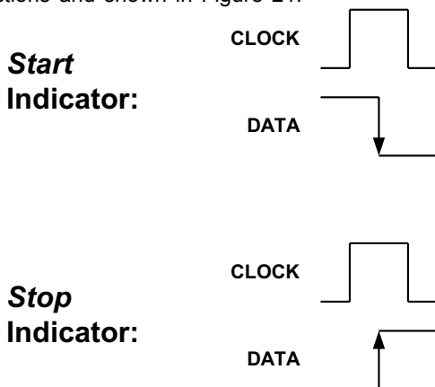
Figure 21: Transmission Indicators
