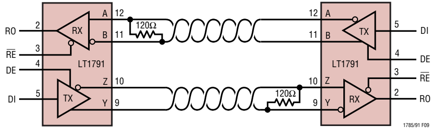
Figure 9. Full-Duplex RS422
