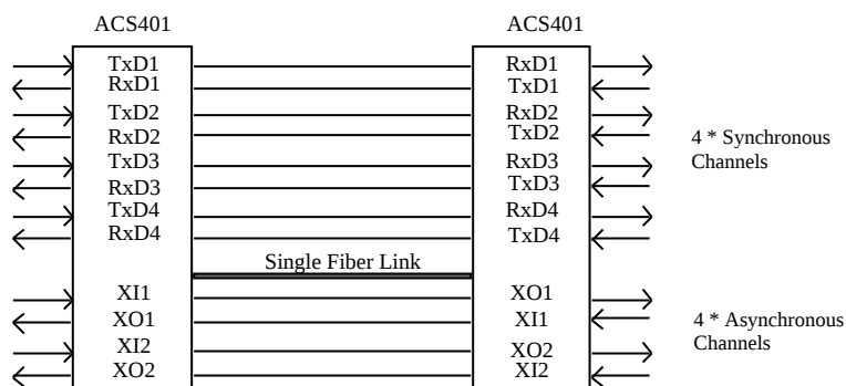
Figure 4. 6 Full-duplex channels over a single fiber
