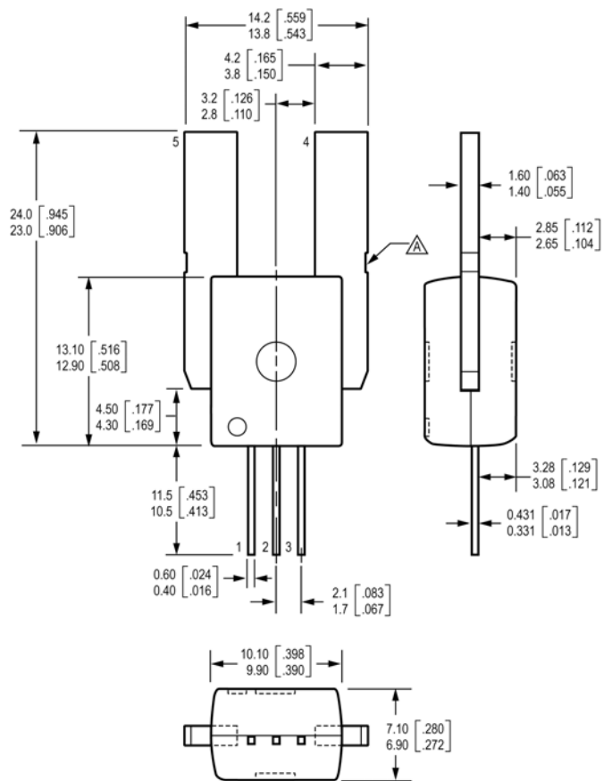
Package CB-PSS
