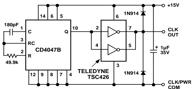
Figure 5. Typical Clock Driver Circuit
