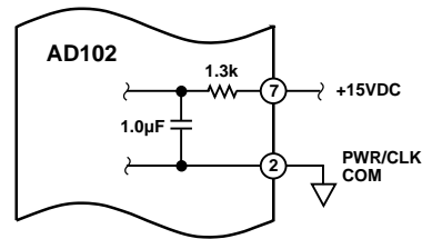
Figure 3. AD102 Power Input
