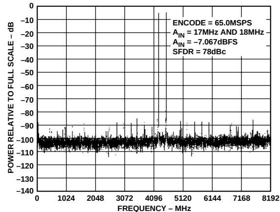
Figure 9. Two-Tone FFT @ 17 MHz/18 MHz
