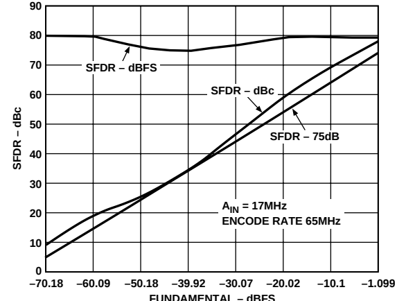
Figure 11. Single Tone SFDR ( A_{IN} @ 17 MHz) vs. Power Level
