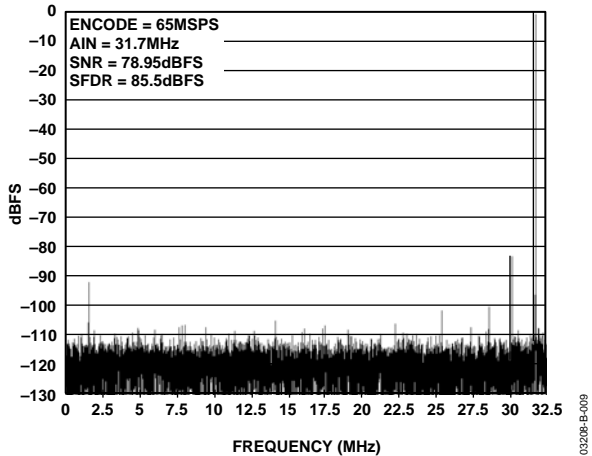
Figure 9. Single-Tone at 32 MHz
