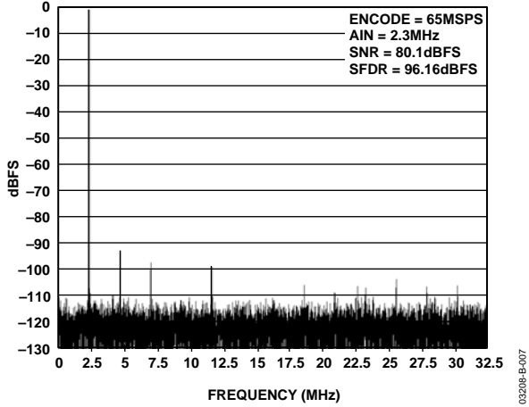
Figure 7. Single-Tone at 2.5 MHz
