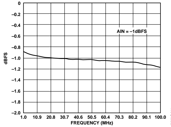
Figure 11. Gain Flatness
