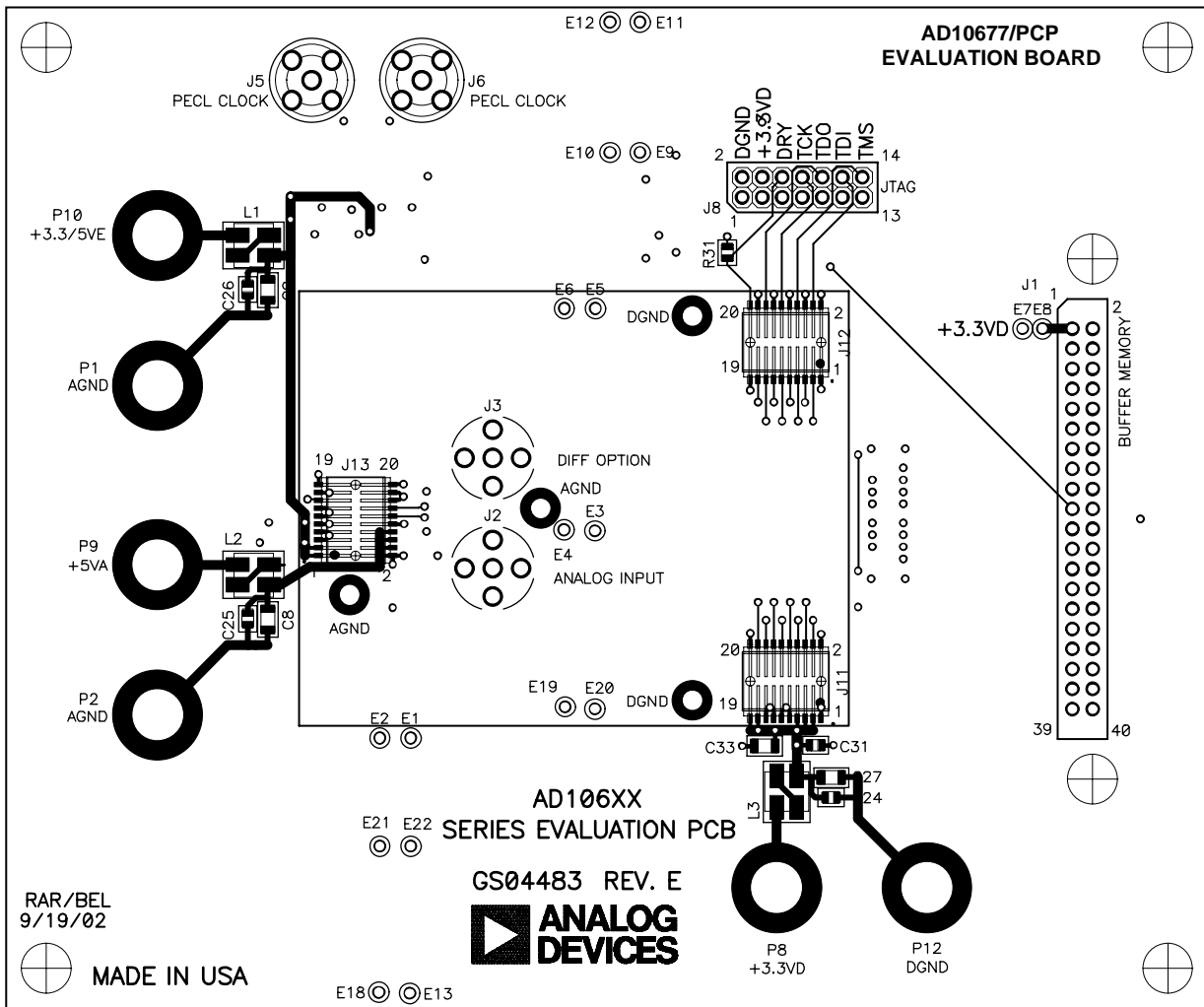
Figure 17. Evaluation Board Mechanical Layout, Top View
