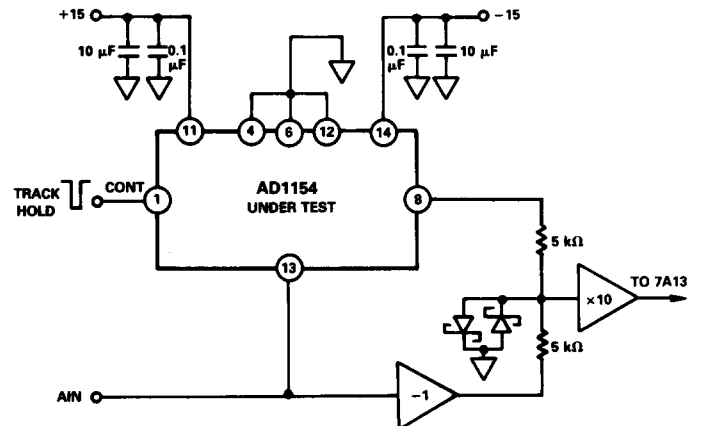
Figure 6. Acquisition Time Test Circuit
