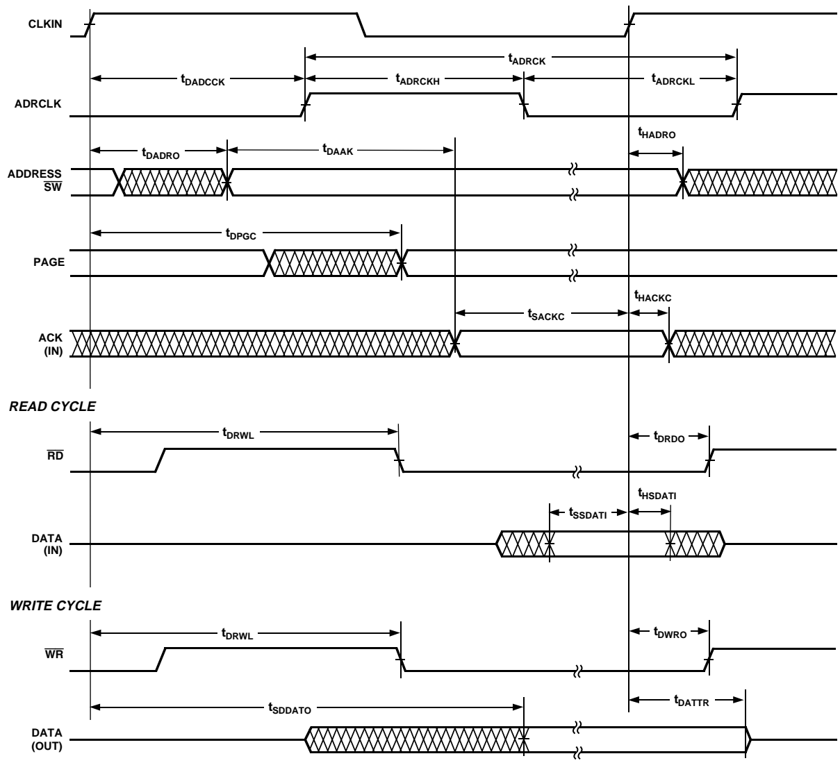
Figure 16. Synchronous Read/Write—Bus Master
