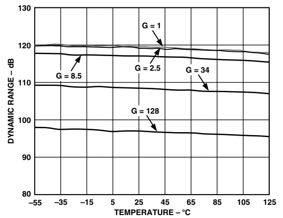
TPC 4. Dynamic Range vs. Temperature
