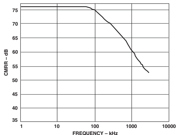
Figure 10. Analog Input CMRR vs. Frequency
