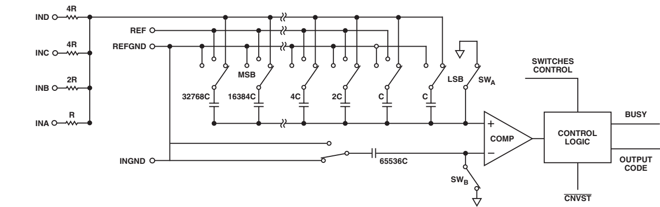
Figure 7. ADC Simplified Schematic
