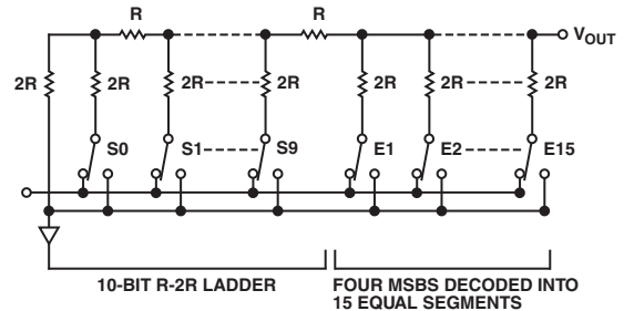
Figure 31. DAC Architecture
