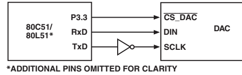
Figure 36. 80C51/80L51 to DAC Interface
