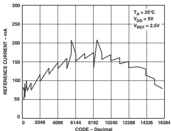
TPC 27. Reference Current vs. Code
