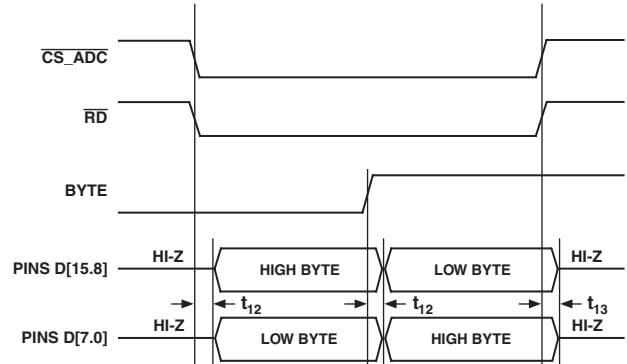
Figure 19. 8-Bit Parallel Interface
