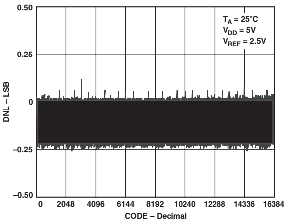
TPC 19. Differential Nonlinearity vs. Code
