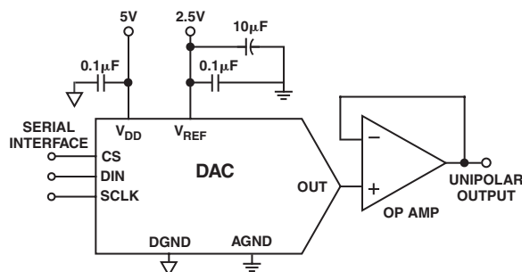
Figure 32. Unipolar Output
