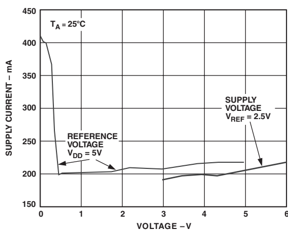
TPC 26. Supply Current vs. Reference Voltage or Supply Voltage
