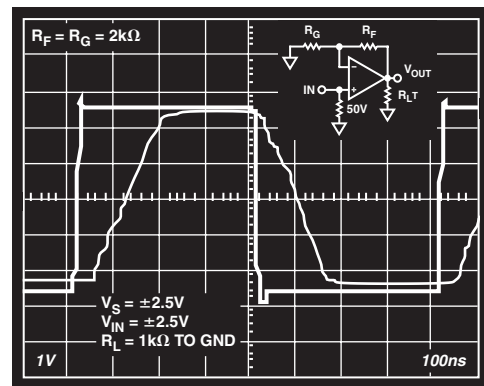
Figure 41. Overdrive Recovery
