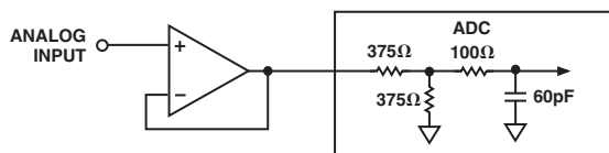
Figure 5b. Analog Input Circuit
