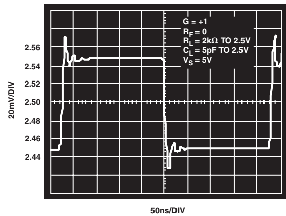
TPC 61. 100 mV Step Response
