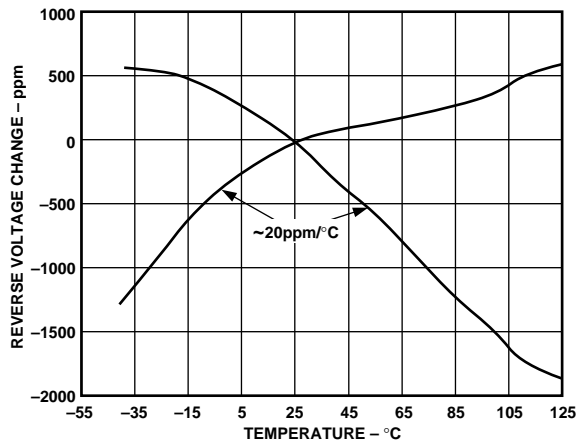
Figure 1. Output Drift for Different Temperature Characteristics
