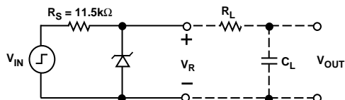
Figure 14b. Turn-On, Settling, and Transient Test Circuit
