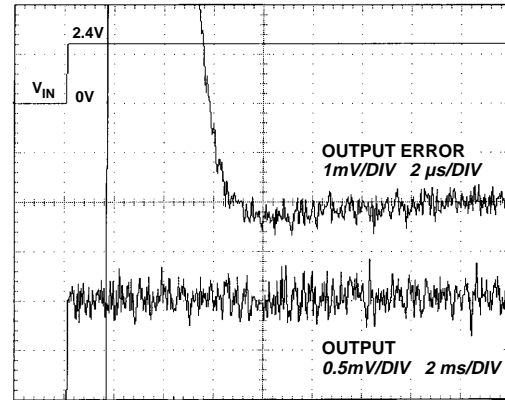
Figure 15. Turn-On Settling
