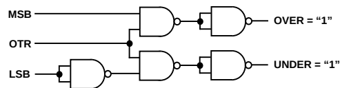
Figure 21. Overrange or Underrange Logic
