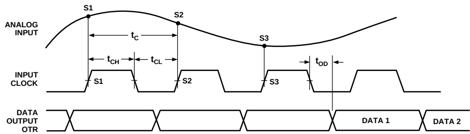
Figure 1. Timing Diagram
