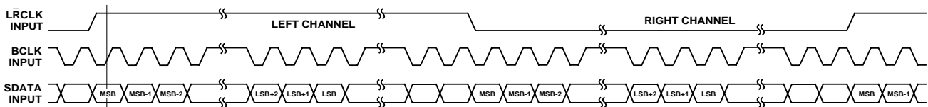
Figure 4. Left-Justified Mode
