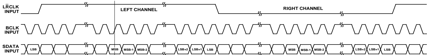
Figure 2. Right-Justified Mode
