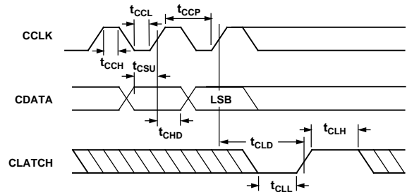
Figure 22. Serial Control Port Timing
