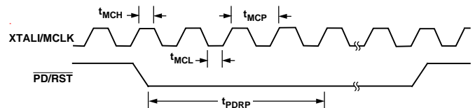
Figure 23. MCLK and Power Down/Reset Timing
