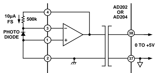
Figure 22. Photodiode Amplifier
