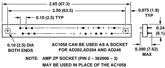
AC1508 Mating Socket
