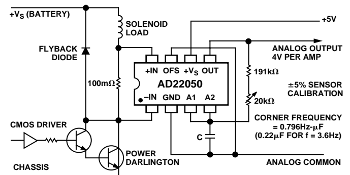
Figure 10. Current Sensor Interface. Gain Is \times 40 , Single-Pole Low-Pass Filtering
