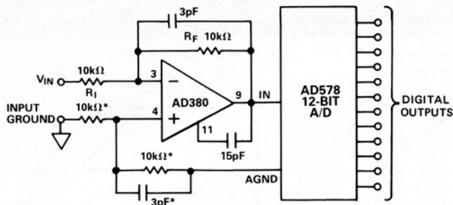
Figure 27. Fast-Settling Buffer
