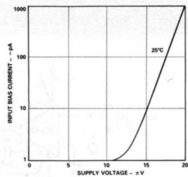
Figure 15. Input Bias Current vs. Supply Voltage
