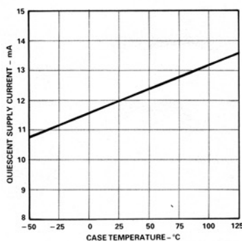
Figure 10. Supply Current vs.
