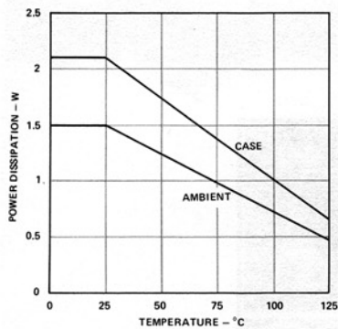
Figure 13. Power Dissipation vs. Temperature
