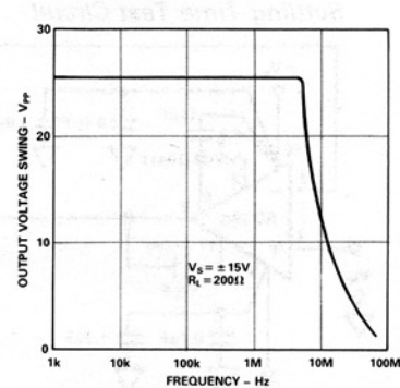
Figure 21. Large Signal Frequency Response
