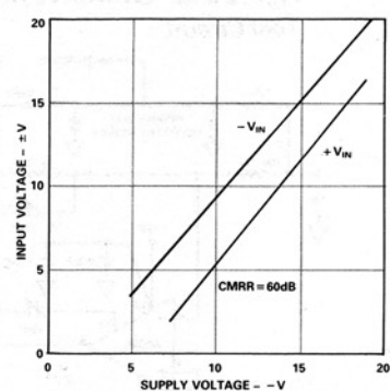
Figure 18. Input Voltage Range vs. Supply Voltage
