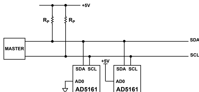
Figure 43. Multiple AD5161 Devices on One I 2 C Bus
