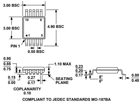
Figure 50. 10-Lead Mini Small Outline Package [MSOP] (RM-10)
