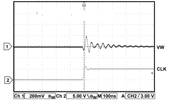
Figure 24. Digital Feedthrough
