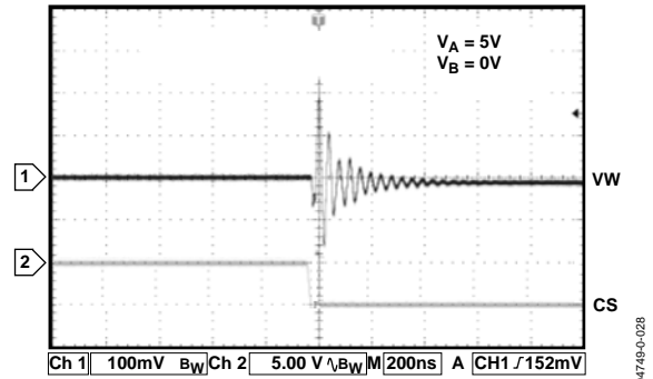
Figure 26. Midscale Glitch, Code 0x80–0x7F
