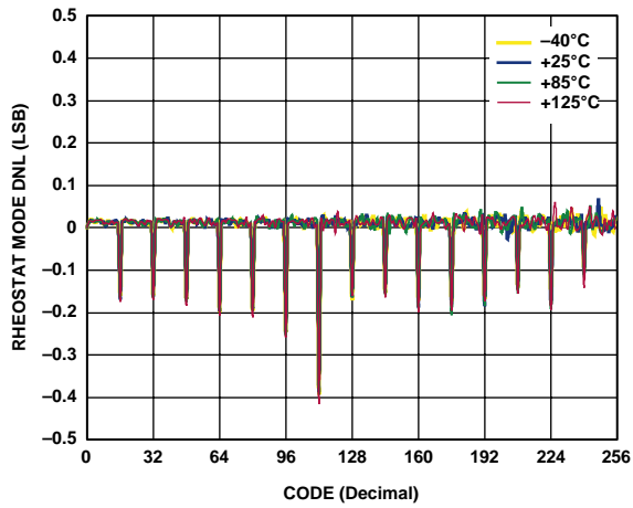
Figure 12. R-DNL vs. Code vs. Temperature, V_{DD} = 5V
