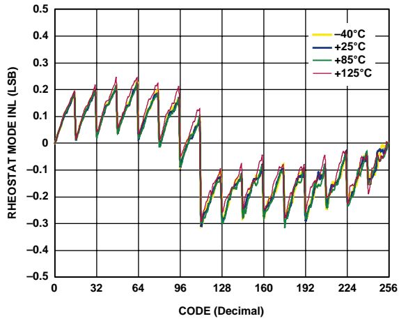
Figure 11. R-INL vs. Code vs. Temperature, V_{DD} = 5V
