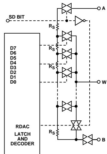
Figure 32. AD5170 Equivalent RDAC Circuit
