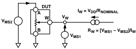
Figure 26. Test Circuit for Wiper Resistance
