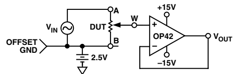
Figure 16. Gain vs. Frequency Test Circuit
