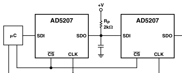
Figure 3. Daisy-Chain Configuration Using SDO
