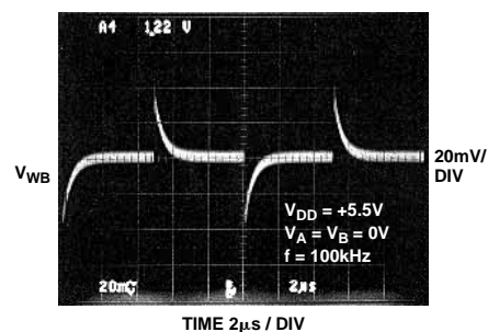
Figure 18. Digital Feedthrough
