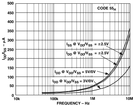
TPC 14. AD5200 10 k \Omega Supply Current vs. Clock Frequency
