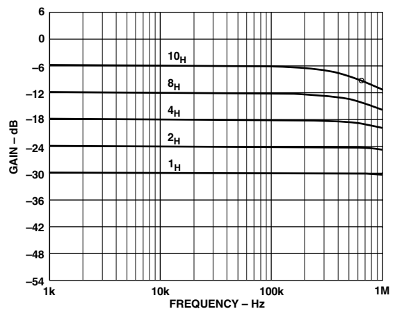
TPC 18. AD5201 10 k \Omega Gain vs. Frequency vs. Code
