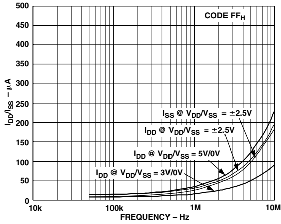
TPC 13. AD5200 10 k \Omega Supply Current vs. Clock Frequency
