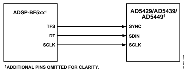
Figure 50. ADSP-BF5xx SPORT-to-AD5429/AD5439/AD5449 Interface
