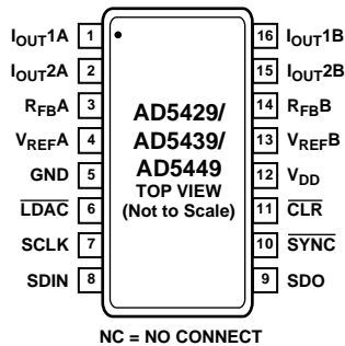
Figure 5. Pin Configuration
