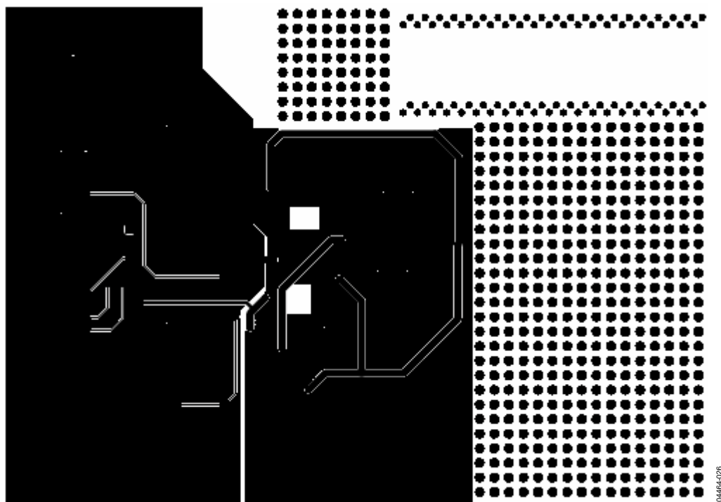
Figure 58. Solder-Side Artwork
