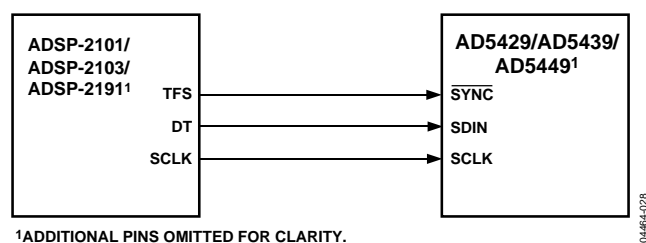
Figure 48. ADSP-2101/ADSP-2103/ADSP-2191 SPORT-to-AD5429/AD5439/AD5449 Interface
