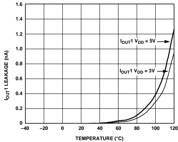
Figure 16. I_{OUT1} Leakage Current vs. Temperature
