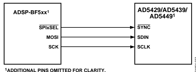
Figure 49. ADSP-BF5xx-to-AD5429/AD5439/AD5449 Interface
