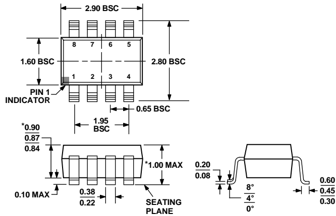
Figure 65. 8-Lead Small Outline Transistor Package [TSOT] (UJ-8) Dimensions shown in millimeters
