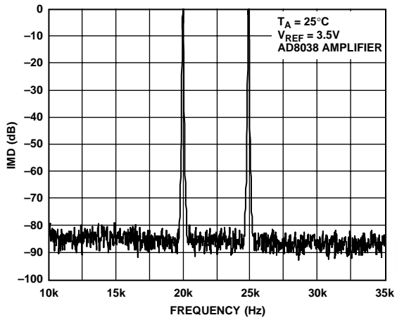
Figure 39. Narrow-Band IMD, f_{OUT} = 20\text{ kHz}, 25\text{ kHz}, \text{Clock} = 1\text{ MHz}
