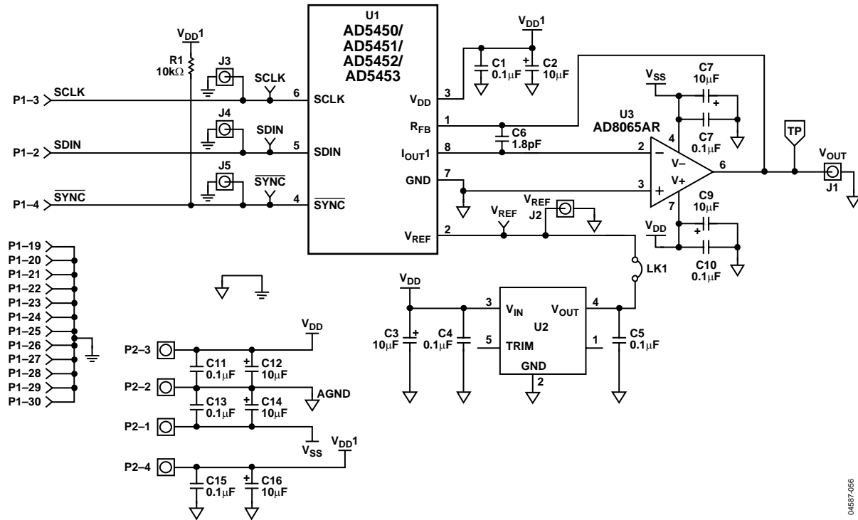
Figure 61. Schematic of AD5450/AD5451/AD5452/AD5453 Evaluation Board
