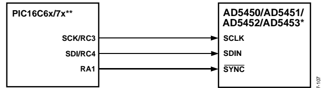
Figure 60. PIC16C6x/7x-to-AD5450/AD5451/AD5452/AD5453 Interface
