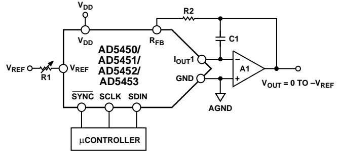
Figure 43. Unipolar Operation
