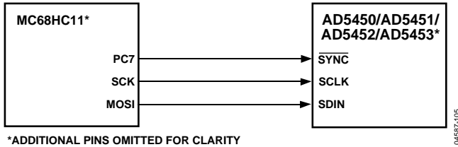
Figure 58. MC68HC11-to-AD5450/AD5451/AD5452/AD5453 Interface
