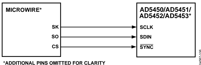
Figure 59. MICROWIRE-to-AD5450/AD5451/AD5452/AD5453 Interface
