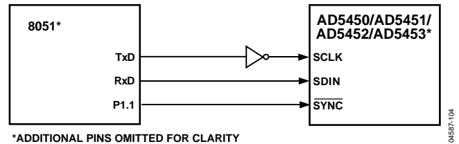
Figure 57. 80C51/80L51 to-AD5450/AD5451/AD5452/AD5453 Interface
