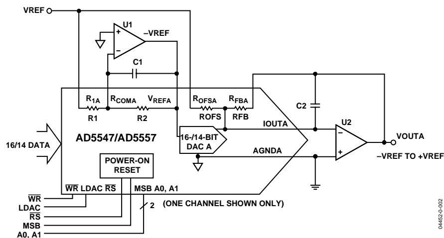
Figure 2. 16/14-Bit 4-Quadrant Multiplying DAC with Minimum of External Components (Only One Channel Shown)
