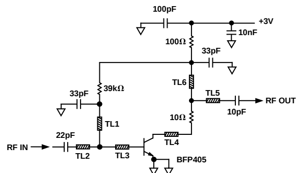
Figure 4. LNA circuit
