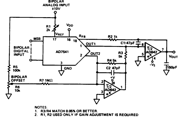
Figure 27a. AD642 Used as DAC Output Amplifier
