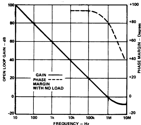
Figure 10. Open Loop
