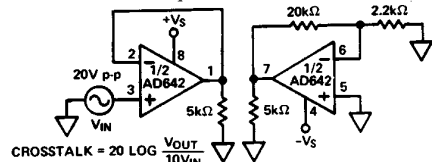
Figure 20. Crosstalk Test Circuit
