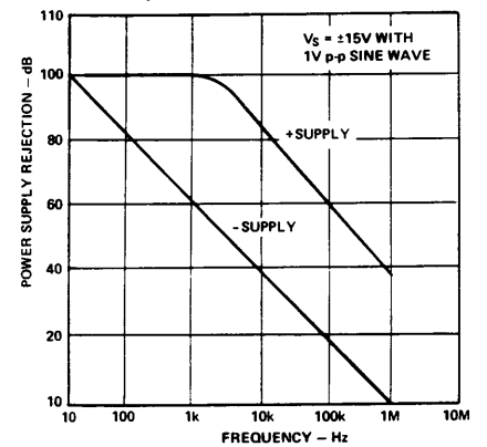
Figure 12. Power Supply Rejection
