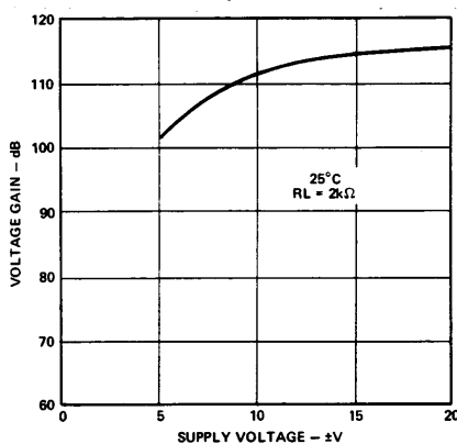
Figure 11. Open Loop Voltage
