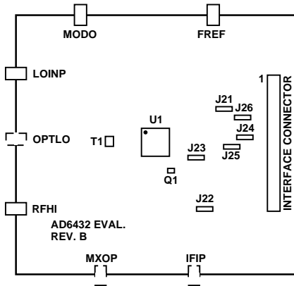
Figure 36. Evaluation Board Layout (Top View)
