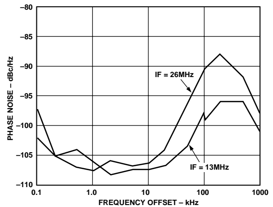
Figure 14. PLL Phase Noise vs. Frequency, V_{POS} = 3\text{ V} , C_{FLTR} = 1\text{ nF} , R_{FLTR} = 1\text{ k}\Omega , F_{REF} = 13\text{ MHz}
