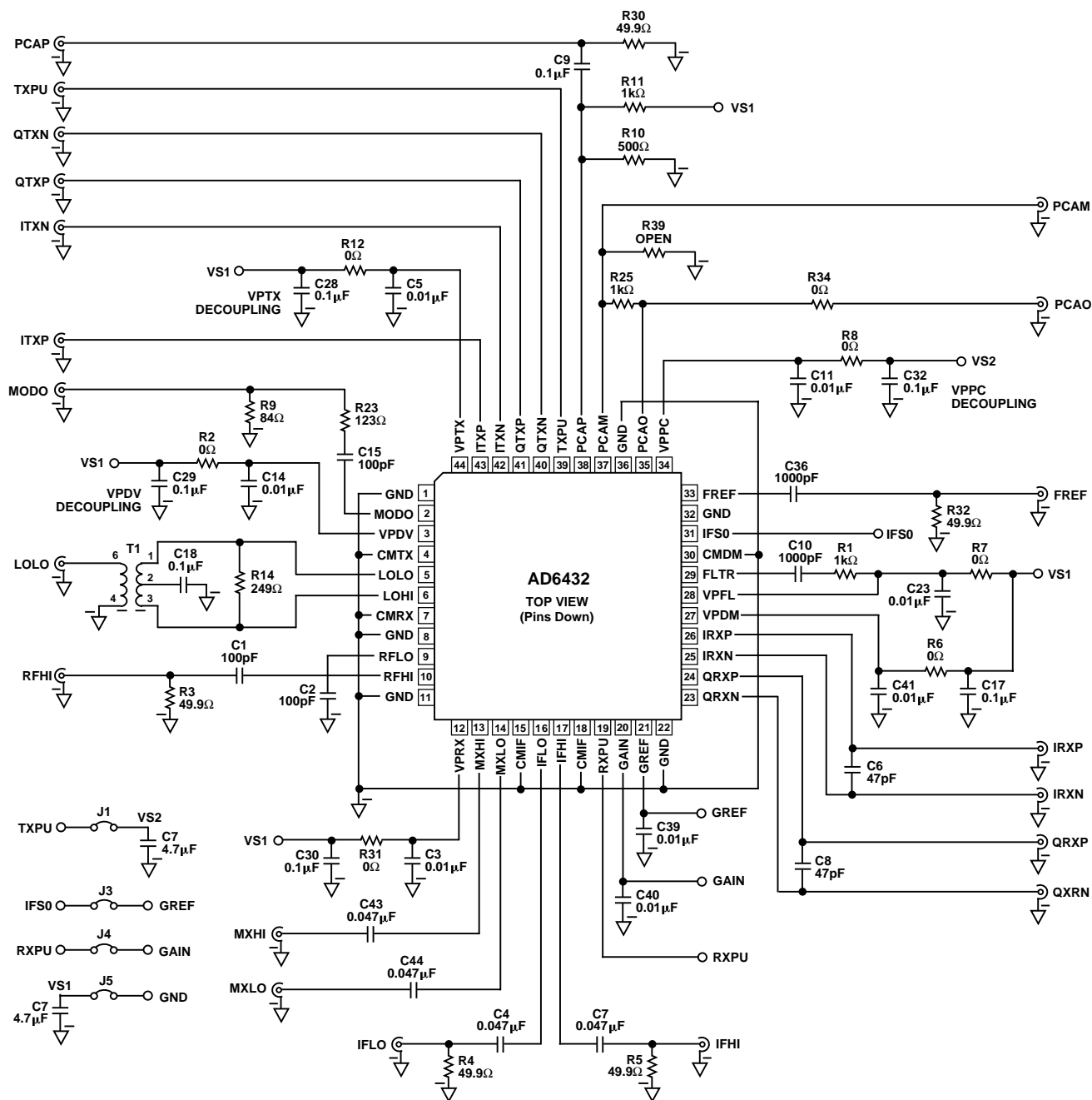
Figure 1. Characterization Board
