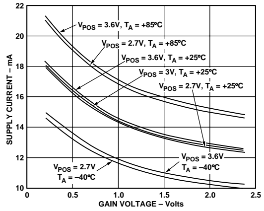
Figure 25. Rx Mode Supply Current vs. V_{GAIN} , V_{GREF} = 1.2\text{ V}
