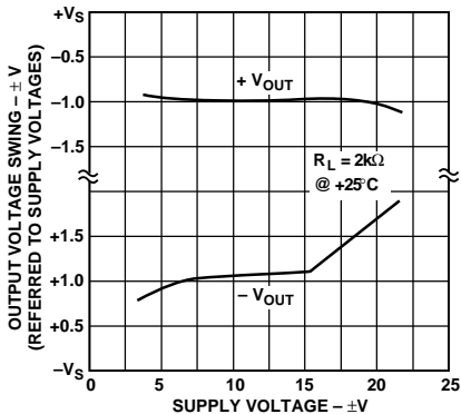
Figure 2. Output Voltage Swing vs. Supply Voltage
