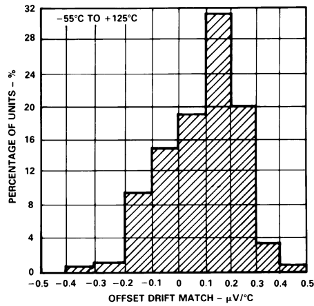
Figure 19. Typical Distribution of Offset Voltage Drift Match
