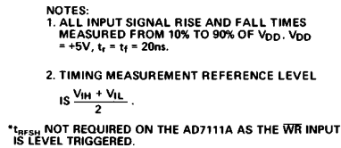
Write Cycle Timing Diagram
