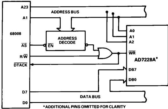
Figure 16. AD7228A to 68008 Interface
