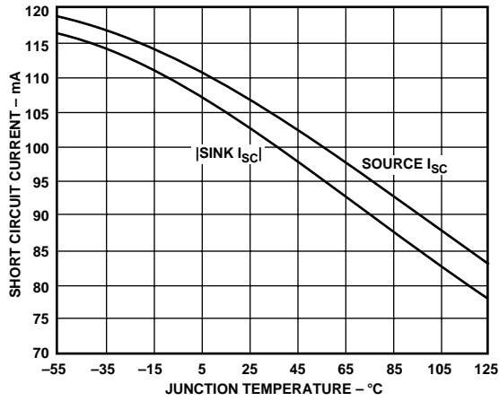
Figure 28. Short Circuit Current vs. Temperature
