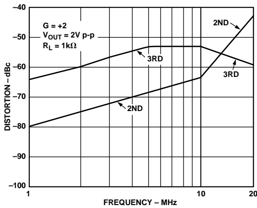
Figure 10. Distortion vs. Frequency; V_S = \pm 5V
