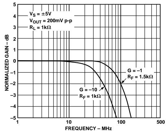
Figure 7. Frequency Response; G = -1, -10 ; V_S = \pm 5 V
