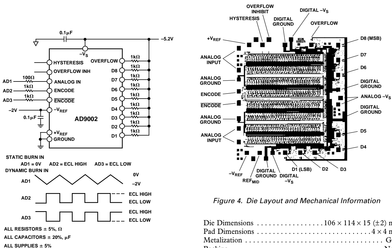
Figure 3. Burn-in Diagram
