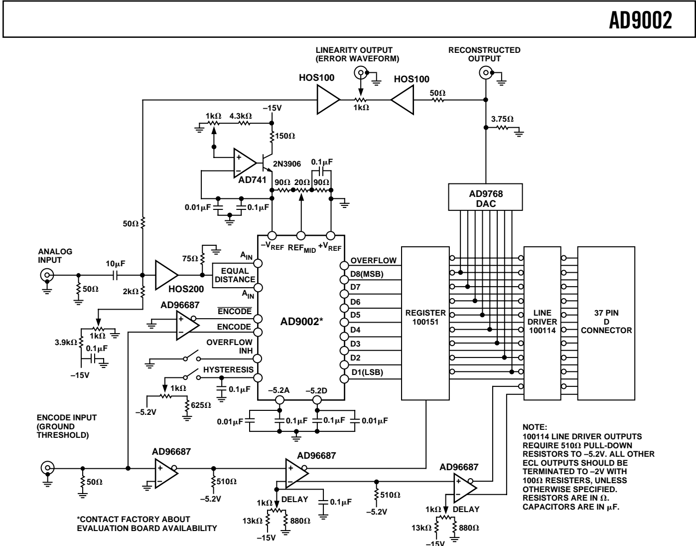
Figure 6. AD9002 Evaluation Circuit
