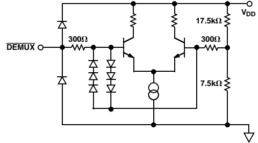
Figure 6. Equivalent \overline{\text{DEMUX}} Input Circuit
