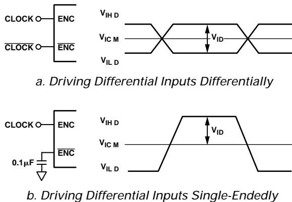
b. Driving Differential Inputs Single-Endedly
