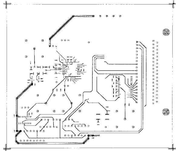
Figure 41. Conductors—Top View
