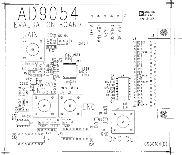
Figure 39. Assembly—Top View
