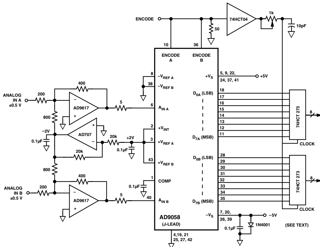
Figure 2. AD9058 Using Internal +2 V Voltage Reference
