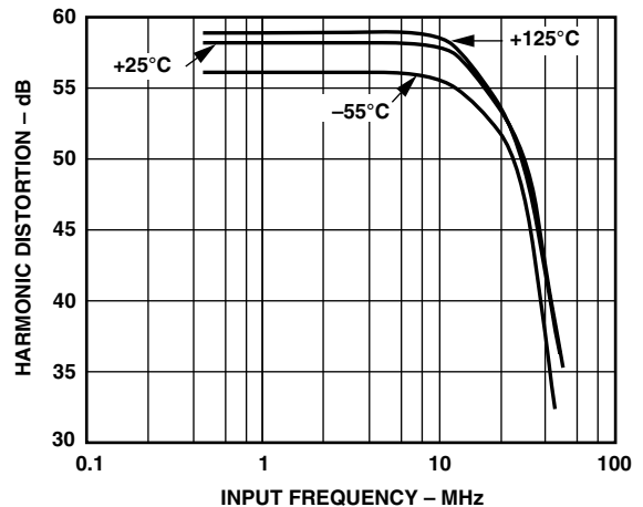
Figure 6. Harmonic Distortion vs. Analog Input Frequency
