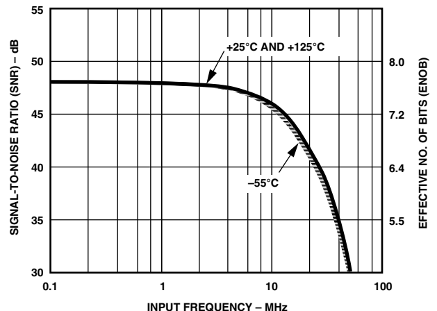
Figure 7. AD9058 Dynamic Performance vs. Analog Input Frequency
