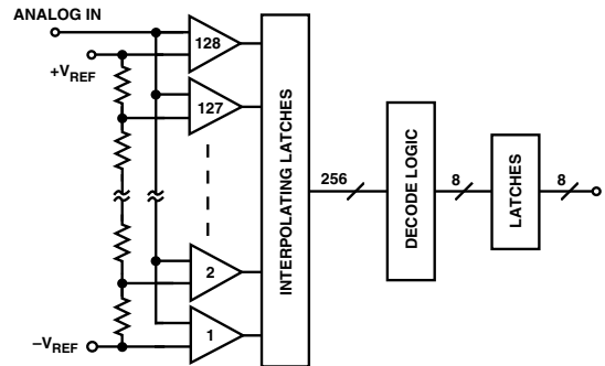
Figure 1. AD9058 Comparator Block Diagram
