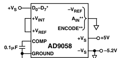
AD9058JD/KD Pinouts
