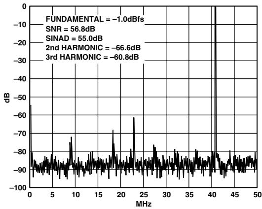
Figure 8. Spectrum: f_s = 100 MSPS, f_{IN} = 40 MHz
