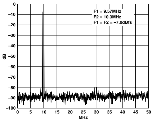
Figure 9. Two Tone Intermodulation Distortion
