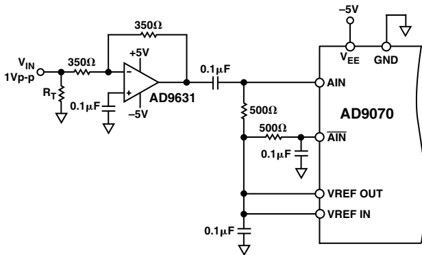
Figure 20. AC-Coupled Input
