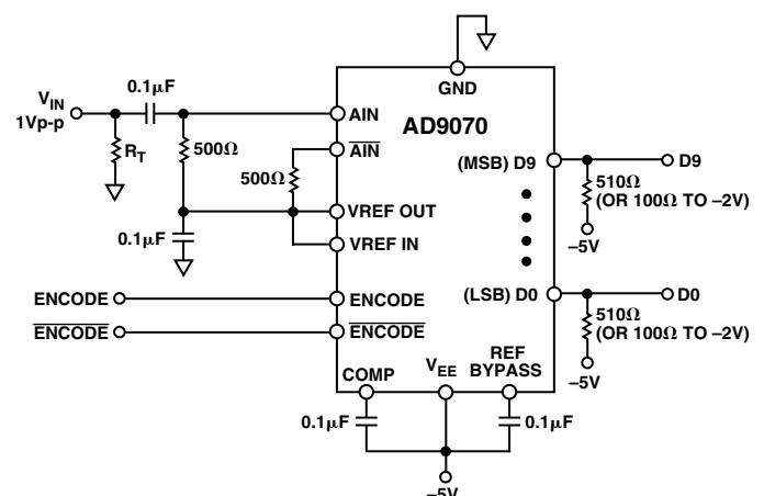
Figure 18. AD9070 in -5\text{ V} (ECL) Environment
