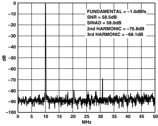
Figure 7. Spectrum: f_s = 100 MSPS, f_{IN} = 10 MHz
