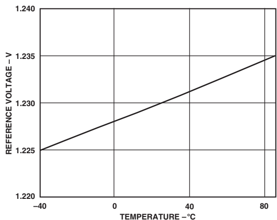
TPC 15. ADC Reference vs. Temperature (with 200 μA Load)
