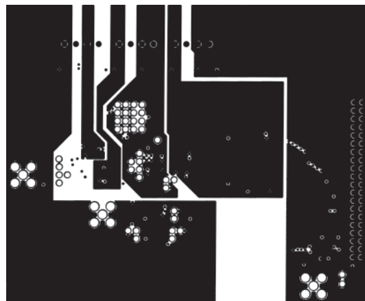
Figure 15. PCB Ground Layer—Layer TBD
