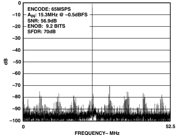
TPC 4. FFT: f_S = 65 MSPS, f_{IN} = 15.3 MHz (2 V p-p) with AD8138 Driving A_{IN}
