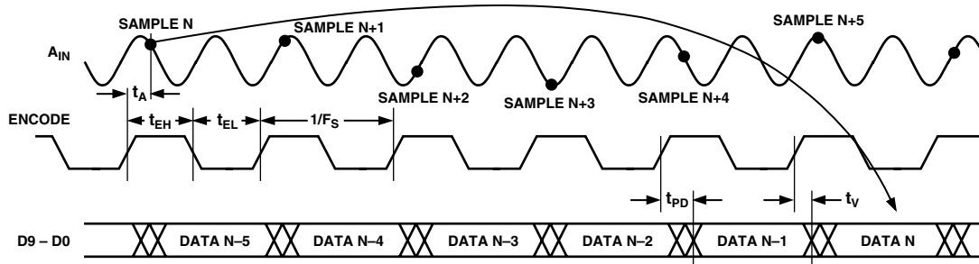
Figure 1. Timing Diagram
