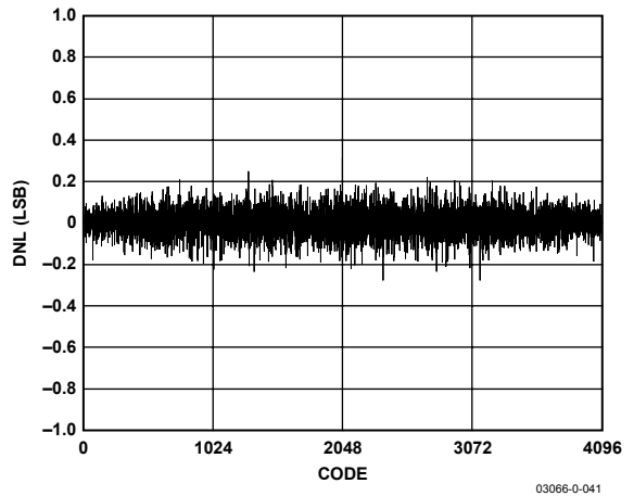
Figure 20. Typical DNL
