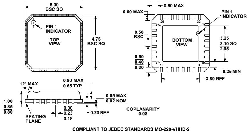
Figure 58. 32-Lead Frame Chip Scale Package [LFCS] (CP-32-1)—Dimensions shown in millimeters
