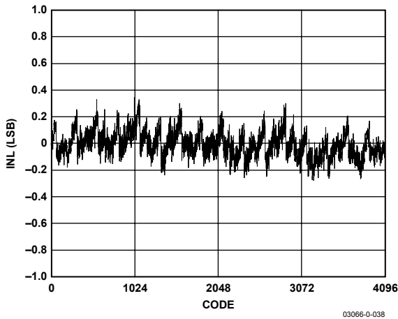
Figure 17. Typical INL
