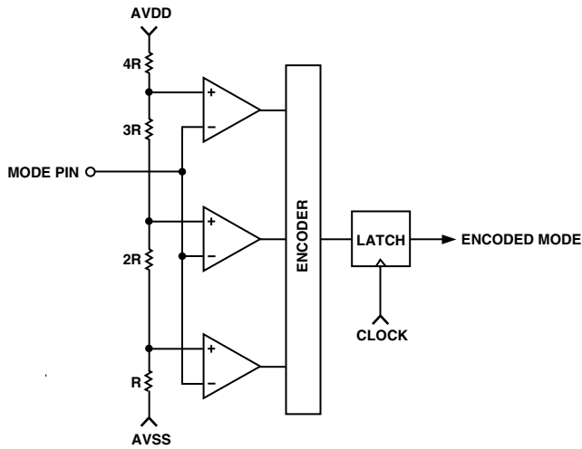
Figure 62. Simplified Mode Pin Circuitry
