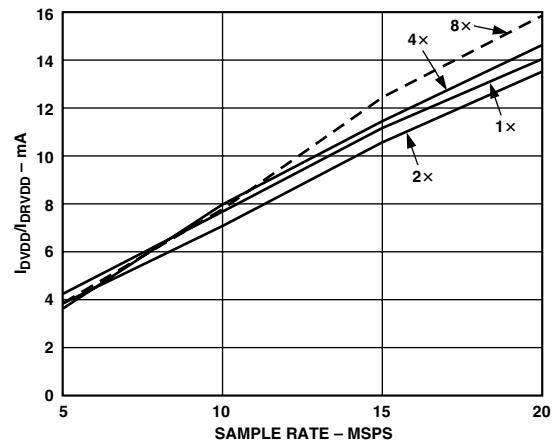
Figure 65a. I_{DVDD}/I_{DRVDD} vs. Sample Rate ( DVDD = DRVDD = 3 V, f_{IN} = 1 MHz)
