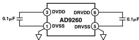
Figure 68. Digital Supply Decoupling
