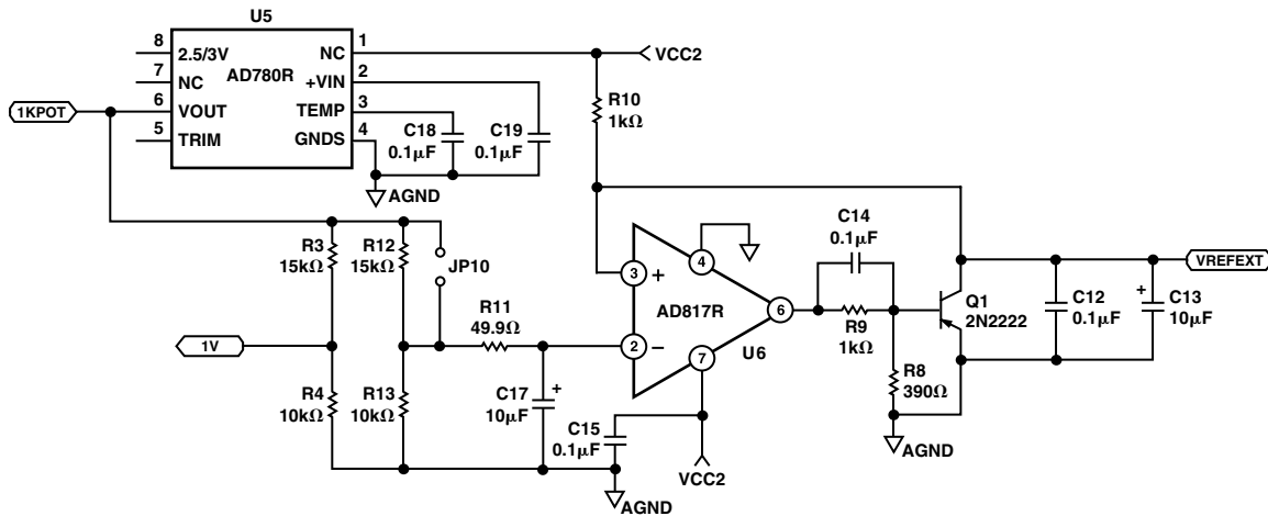
Figure 70. Evaluation Board External Reference Circuitry
