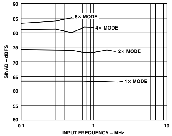
Figure 14. SINAD vs. Input Frequency ( f_{\text{CLOCK}} = 10 MSPS) 1
