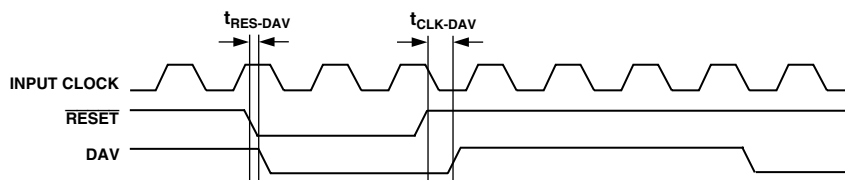
Figure 4b. RESE̅T Timing Diagram
