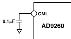
Figure 59. CML Decoupling
