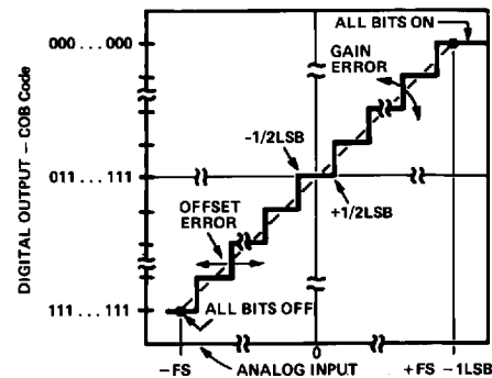
Figure 4. Transfer Characteristics for an Ideal Bipolar A/D
