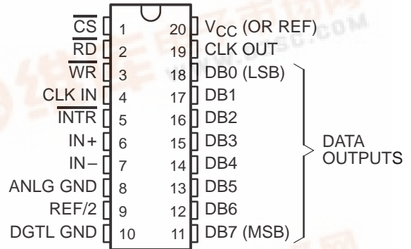
N PACKAGE (TOP VIEW)
