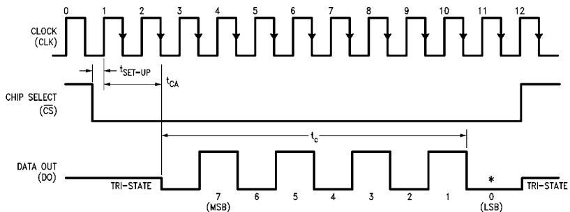
ADC08231 Timing
