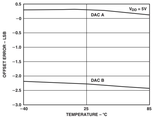
TPC 3. Offset Error vs. Temperature
