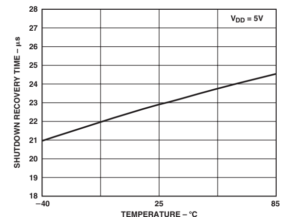
TPC 9. Shutdown Recovery Time vs. Temperature
