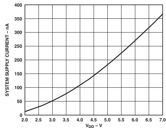
TPC 8. System Supply Current at Shutdown
